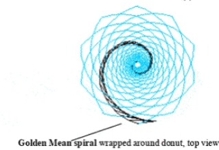
Golden Mean spiral wrapped around donut, top view
